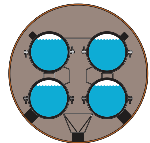
Fig 2. Multi-pipe casing spacer with four carriers in one casing.
